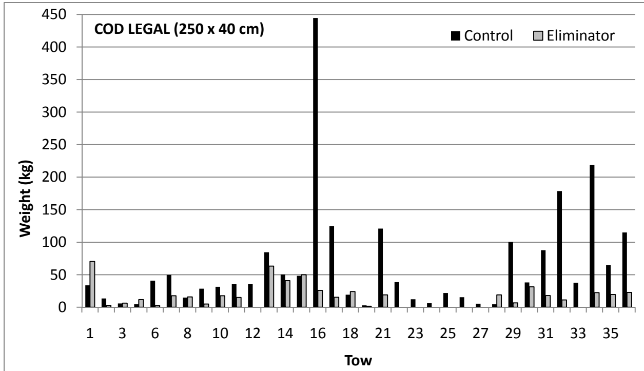
Figure A3. Legal cod in kg by tow in the 250 x 40 cm Eliminator Trawl™.
