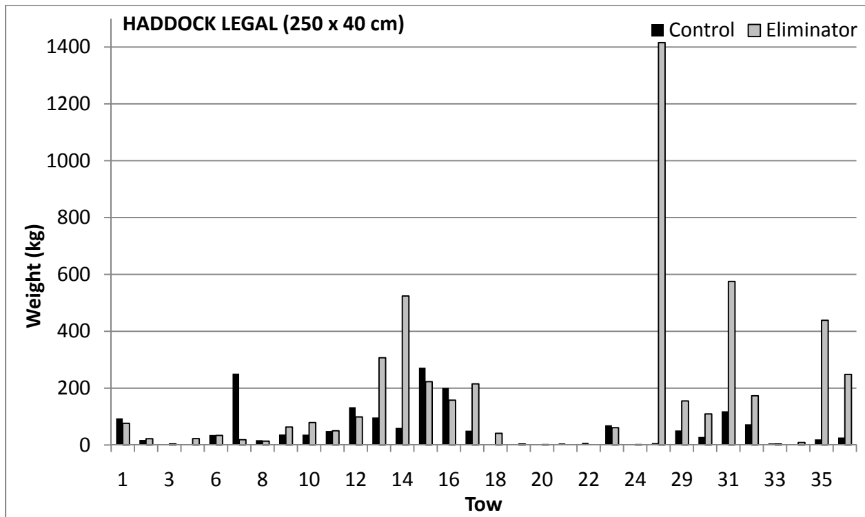
Figure A4. Legal haddock in kg by tow in the 250 x 40 cm Eliminator Trawl™.
